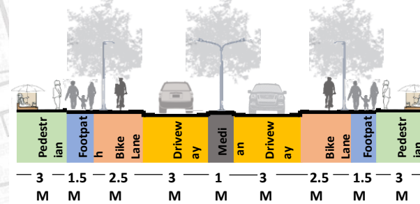
Section -15M wide road
